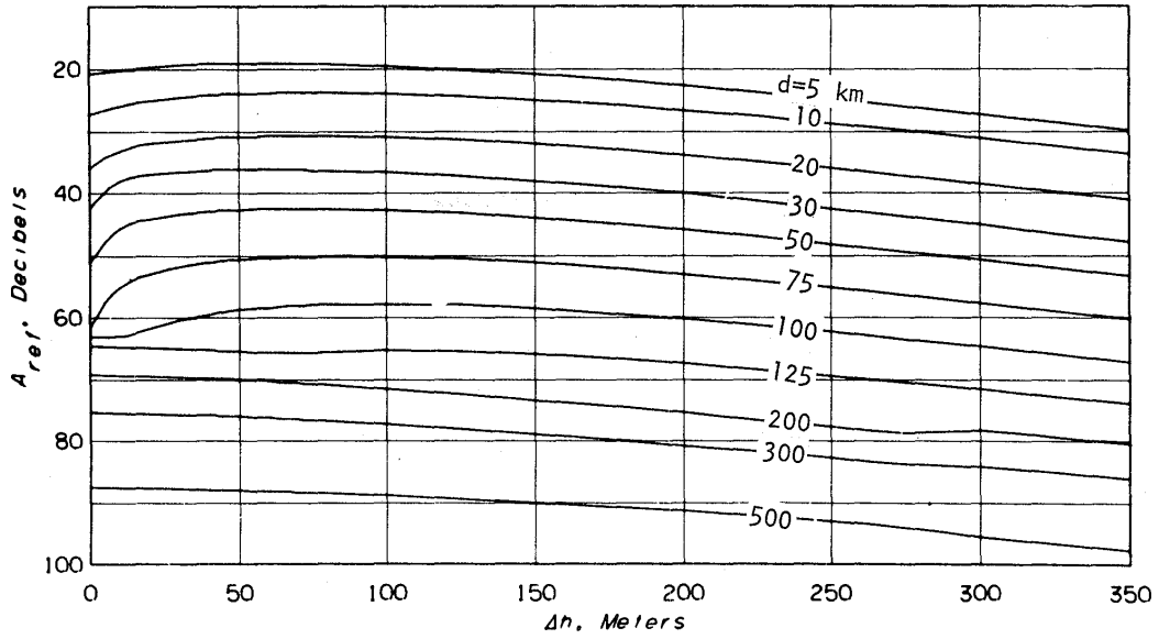
(a) f = 150 MHz, h_{g1} = 30 m, h_{g2} = 2 m
