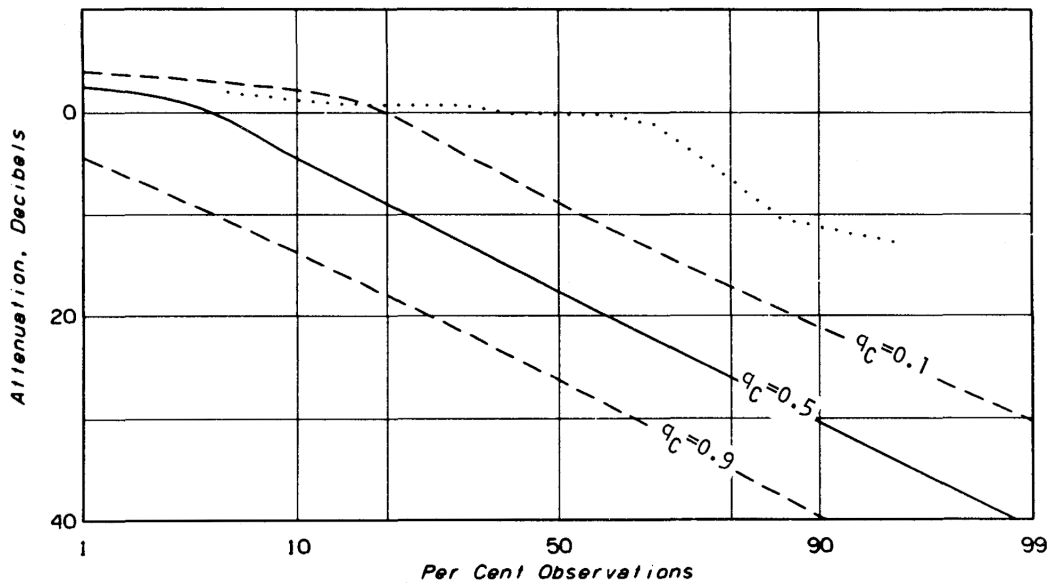
(b) Distance, about 50 km; 11 points.
