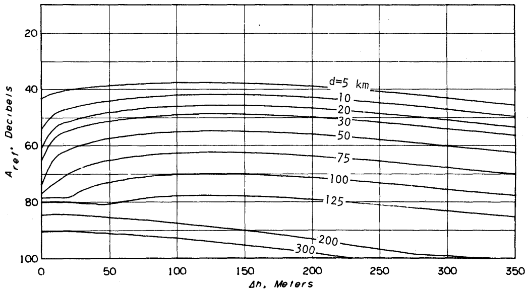
(b) f = 150 MHz, h_{g1} = 2 m, h_{g2} = 2 m
