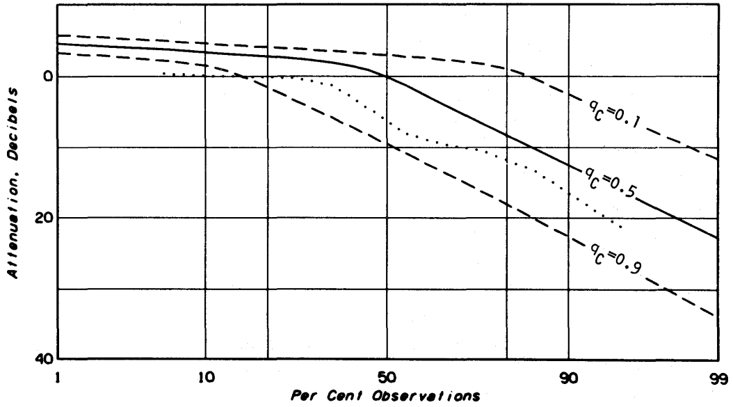
(a) Distance, about 20 km; 10 points.
