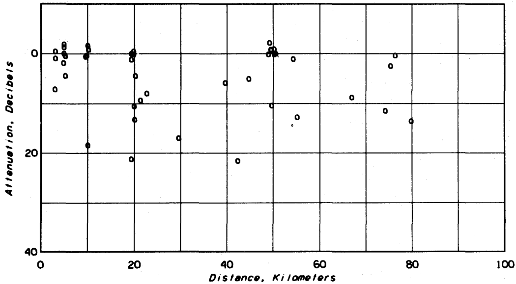
Figure 8: The R3 data at 410 MHz; 44 points.
