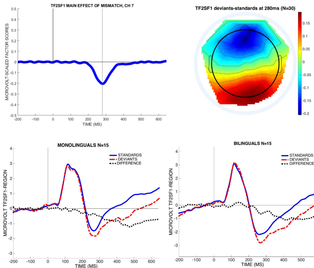
Fig. 5. Upper panel: Main effect factor waveform for the first negative peak and spatial distribution of this effect in the factor. Lower panel: mean waveforms for each child group for standard and deviants computed for the region in blue in the topographical plot.
