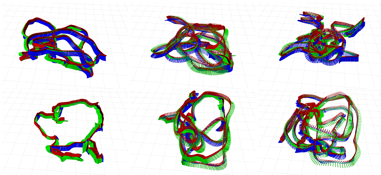
Figure 4: Example generated trajectories on the EuRoC MAV dataset.
