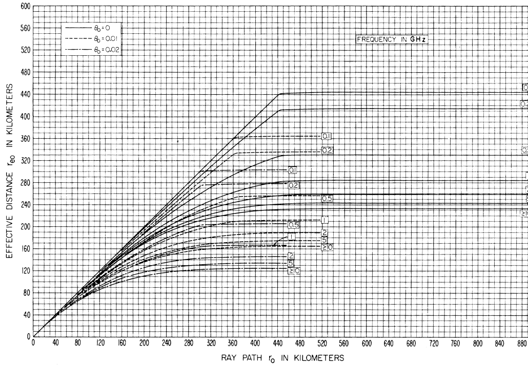
EFFECTIVE DISTANCES r_{eO} AND r_{eW} FOR ABSORPTION BY OXYGEN AND WATER VAPOR \theta_0 = 0, 0.01, 0.02
