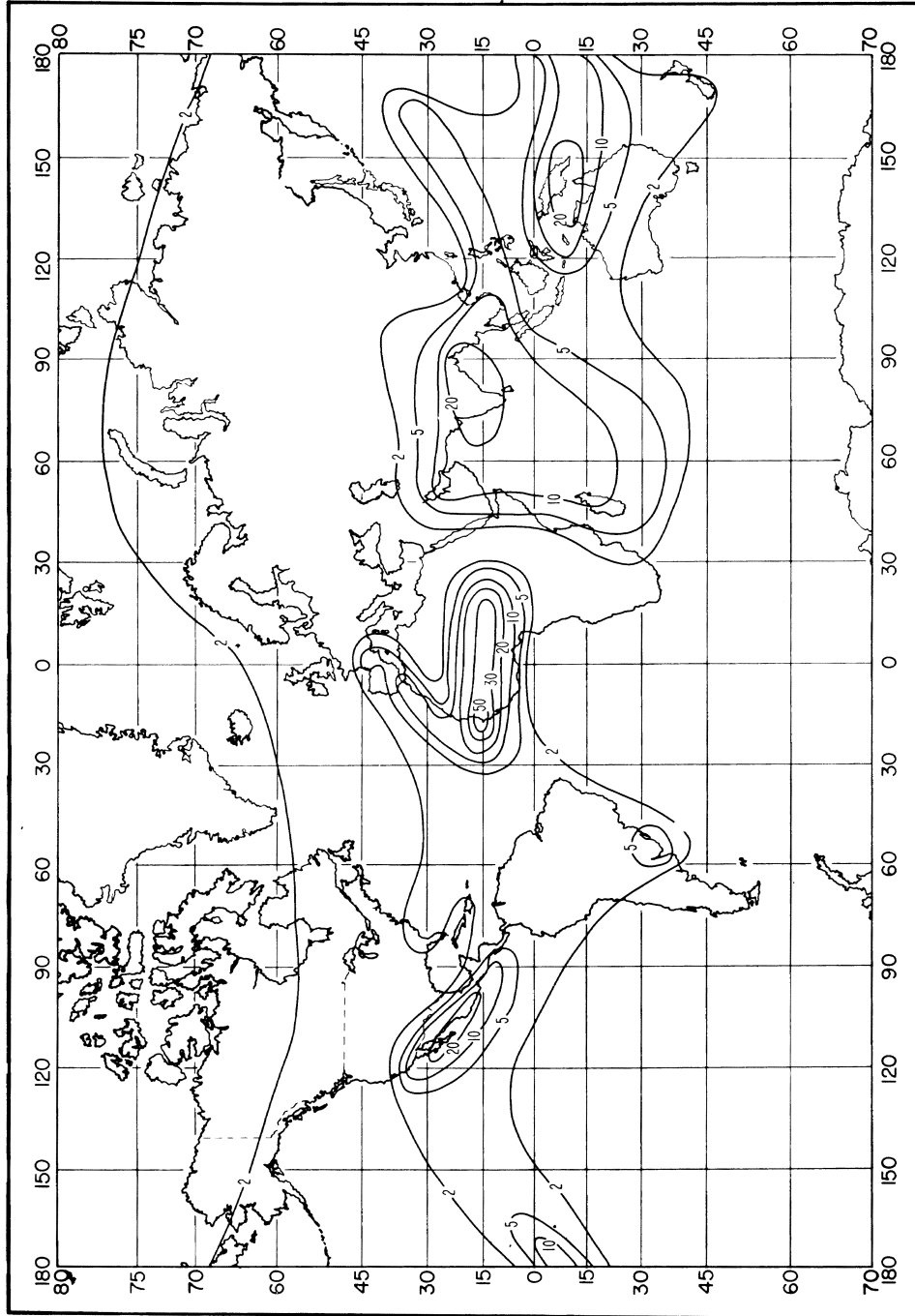
Percent of Time Trapping Frequency is Less Than 3000 MHz: February
