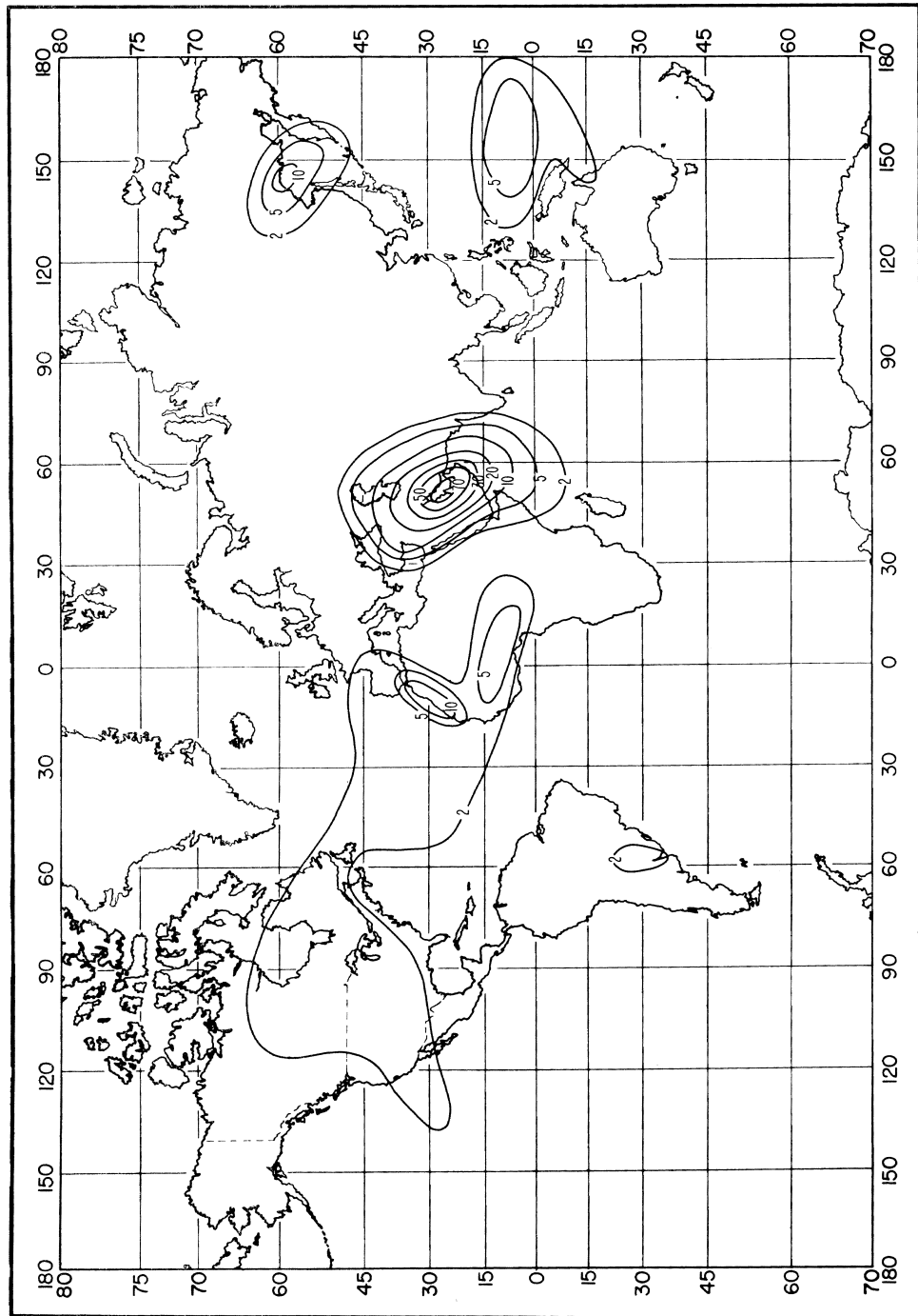
Percent of Time Trapping Frequency is Less Than 300 MHz: August
